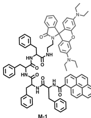
Scheme 1. Structure of M-1 .
